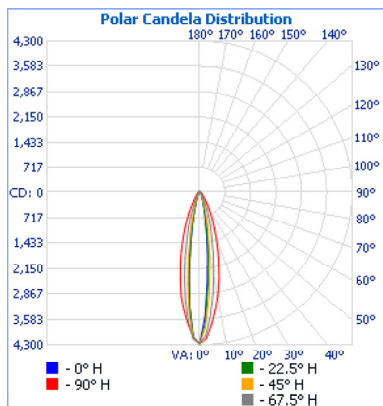
LZWET-1-UNV-840-11L-1525-LD.ies
