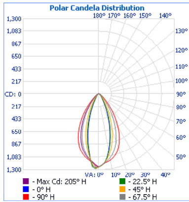
LZWET-1-UNV-840-11L-3060-LD.ies
