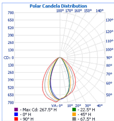
LZWET-1-UNV-840-11L-5080-LD.ies
